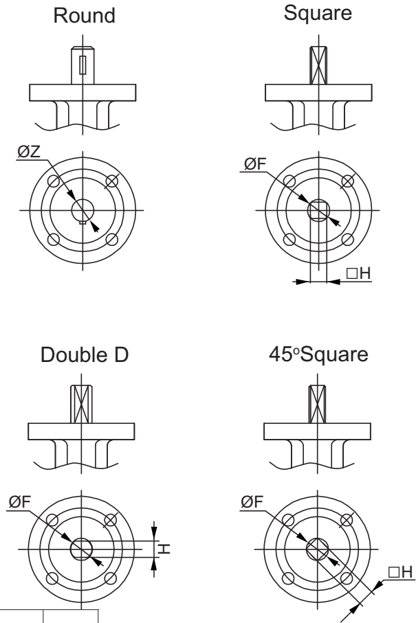
DN40-DN300 B10 Lug Type Butterfly Valve Two Shafts
